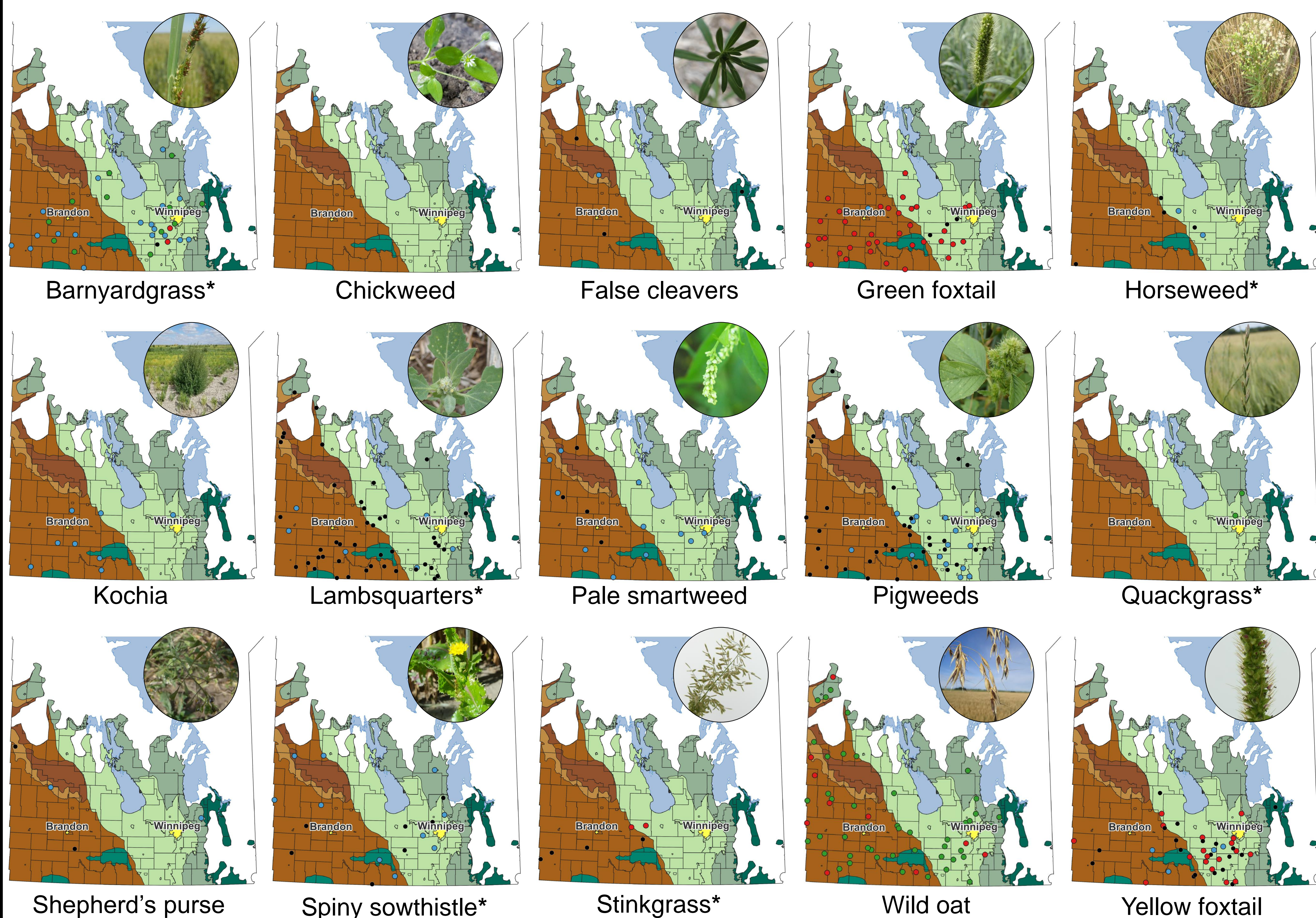
Figure 3. Maps showing the locations of populations exhibiting resistance to acetyl-CoA carboxylase (ACCCase)-, acetolactate synthase (ALS)-, and ACCCase + ALS-inhibiting herbicides for each weed species with resistant biotypes in a 2022 survey of 155 fields in Manitoba.
